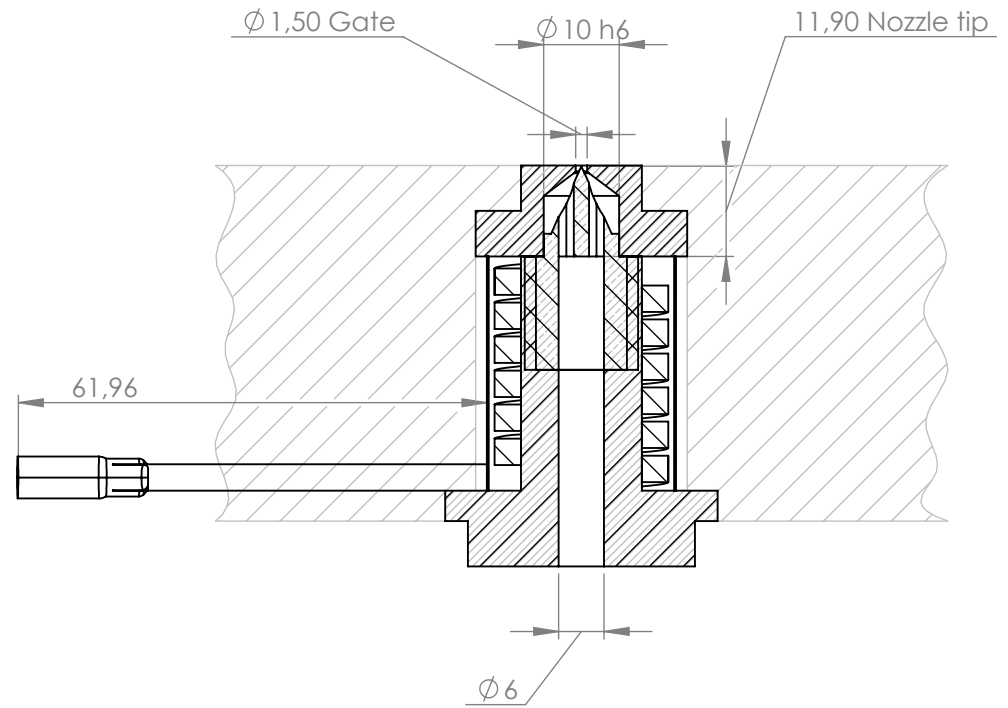
SECTION A-A SKETCH FOR INSTALATION
