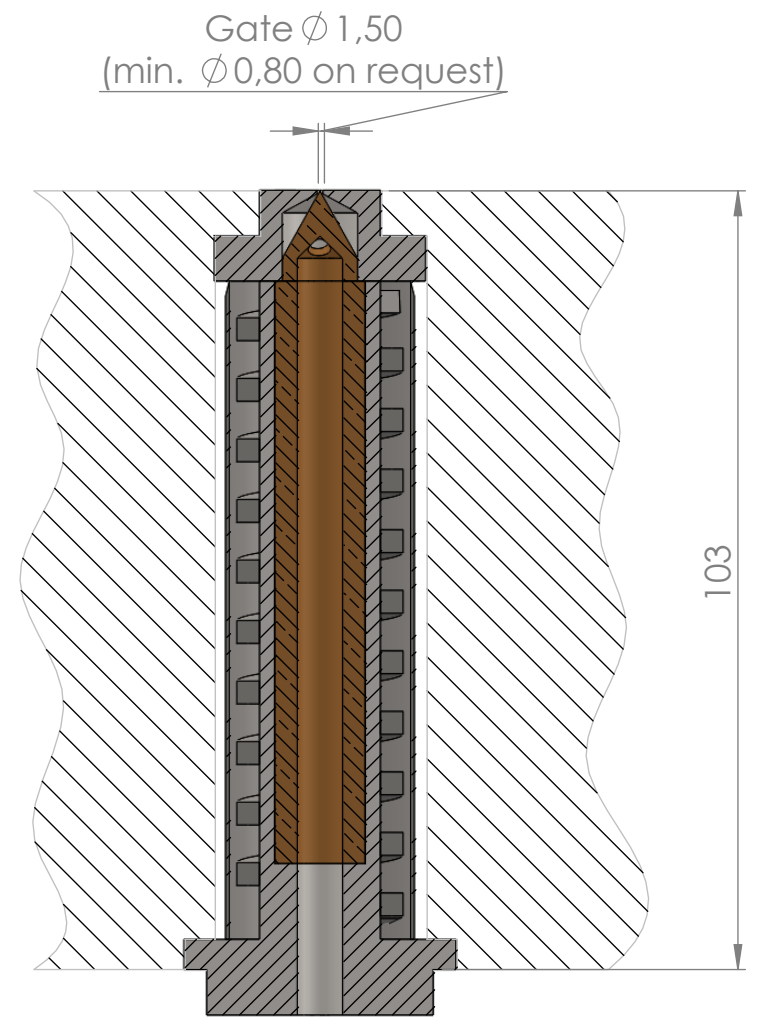
SECTION A-A SKETCH - BUILT IN MOLD
